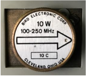
10watt scale
